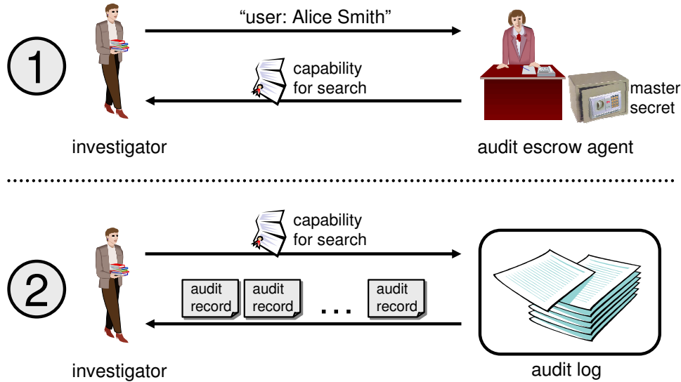
Figure 2. Searching the log: First, the investigator has to obtain a search capability for the keyword in question. Then, she can search the audit log for that keyword.
